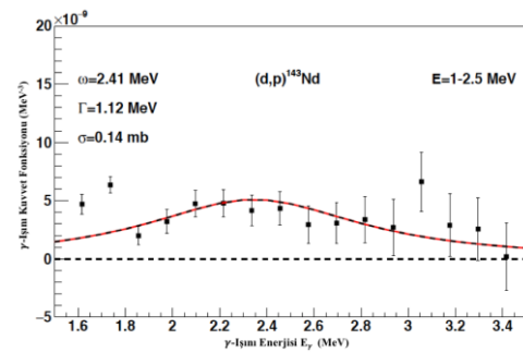
^{143}\text{Nd}
